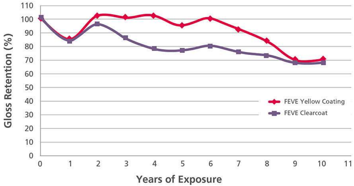
FIGURE 10 » Florida weathering gloss retention.
