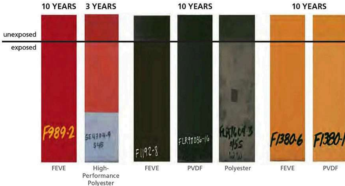
FIGURE 9 » Florida weathering.
