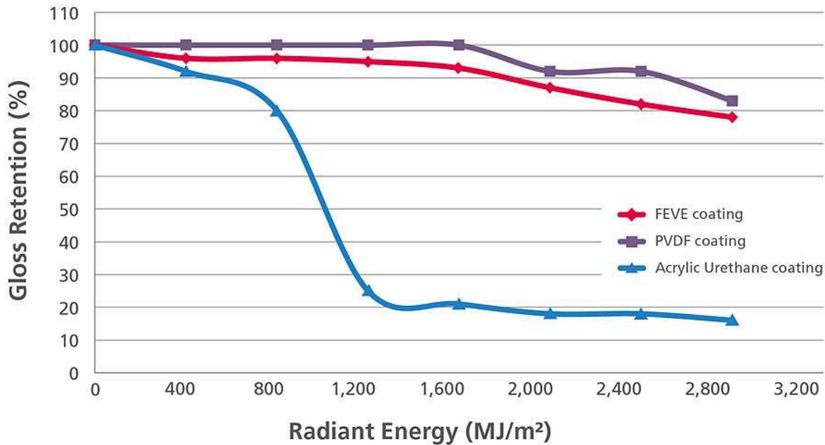
FIGURE 8 » EMMAQUA testing.
