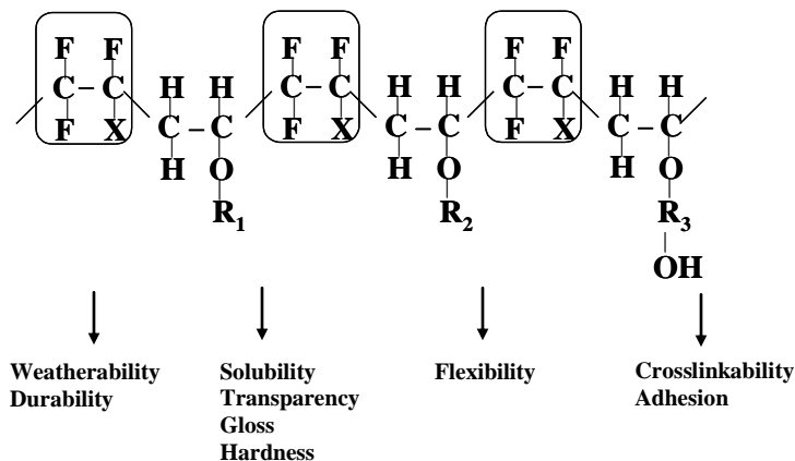
Figure 1. Polymer Structure of FEVE Copolymer
