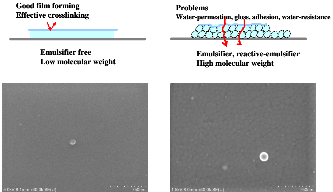
Figure 5. Scanning Electron Micrographs of Films of FEVE Dispersion and Emulsion
