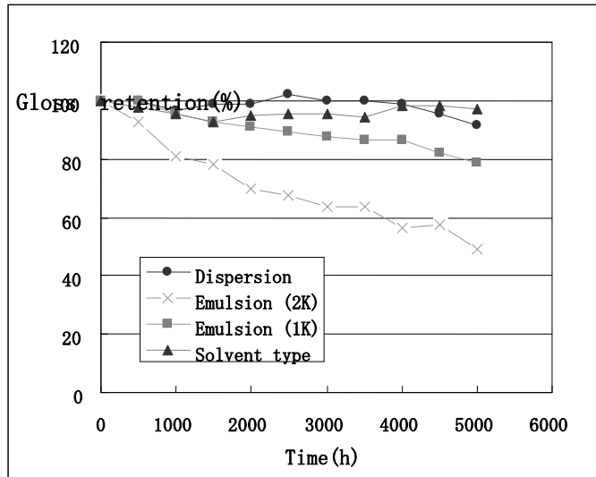
Figure 4. Accelerated Weathering Test Results (QUV)
