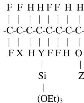
Figure 8: Silanol Functional FEVE Resins
