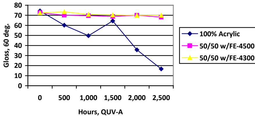
Figure 7: FEVE Resin Blends with Acrylic Resin #2
