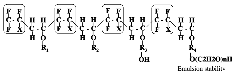
Figure 2: Polymer Structure of FEVE Emulsion
