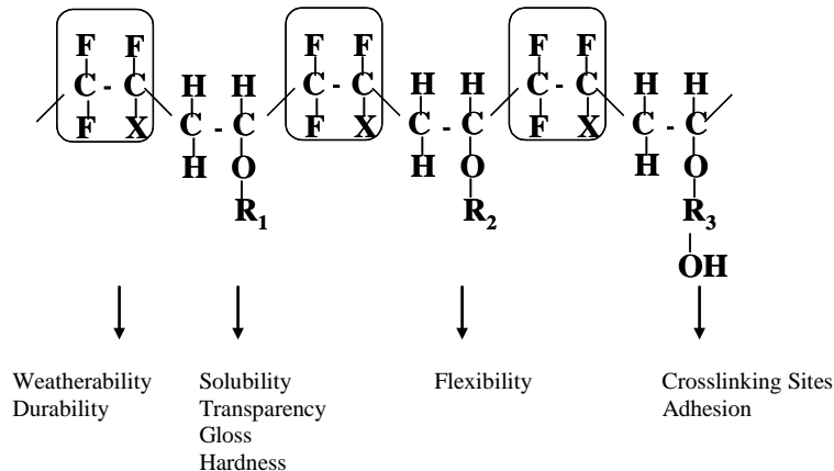
Figure 1: Chemical Structure of FEVE Resin
