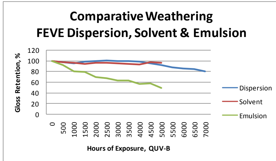
Figure 4: QUV-B Weatherometer Testing of FEVE-Based Coatings
